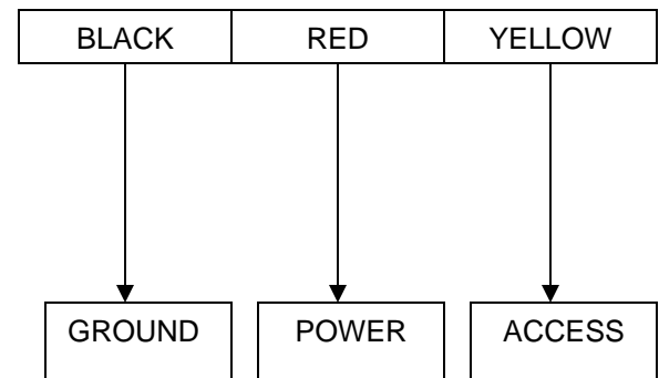
8.1 – Wiring Requirements
