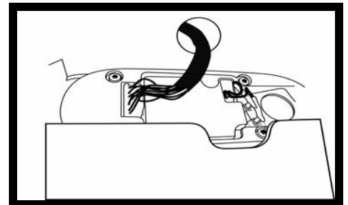
4.1 – Opening cut out of back for wiring to pass through
